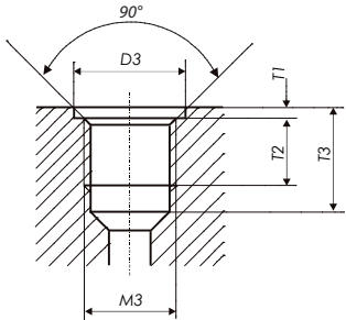
Screw-in hole according to ISO 9974-1 and DIN 3852 Part 1, Form X for screw-in pins Form A, B, and E
